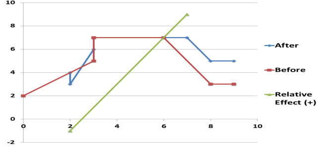
Figure 3: Update timeline \mu_3 of real variable z w.r.t. effect \langle z += (2, -1), [2, 7] \rangle , denoted by the green (line) segment, during and after its interval (Example 1). The red segments represent timeline \mu_3 and the blue ones denote the new i-literals in the resulting timeline. The value of z over [0, 2) (before the effect) remains unchanged. The value of z at time 2 reduces by 1 (adds -1 ) from 4 to 3 and then continuously changes with the combined rate 1 + 2 = 3 to 6 at time 3. It then remains unchanged over the fixed points [3, 6) , despite the effect in this interval. Over the rest ( [6, 7) ) of the interval of the effect, z changes with the combined rate -2 + 2 = 0 from value 7 (i.e., it remains unchanged over [6, 7) ). Since z increases by 2 by the effect at its right endpoint 7, it increases by 2 for all time points after 7 (and before any fixed point after 7). This results in two i-literals \langle z = (-2, 7), [7, 8] \rangle and \langle z = 5, [8, \infty) \rangle above their predecessors \langle z = (-2, 5), [7, 8] \rangle and \langle z = 3, [8, \infty) \rangle .
