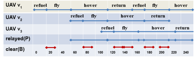
Figure 1: An example of a solution for three UAVs to continuously relay a VIP P , where t_r = 20 (refueling time), t_g = 60 (required start-by time), and t_l = 200 (required duration of relay), assuming each UAV can fly and/or hover for at most 140 time units.
