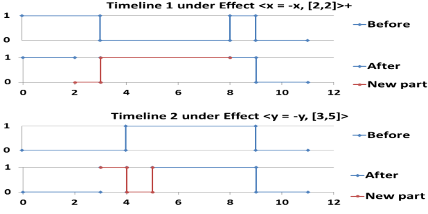
Figure 2: Update timelines \mu_1 & \mu_2 of binary variables w.r.t. the first two effects (Example 1, presented later) following rule 5. The extendable effect \langle x = \neg x, [2, 2]^+ \rangle flips (the value of) x at time 2 of \mu_1 and extends this value until the next effect starts at time 3. Then it flips x from time 3 and before the fixed point 8 of absolute effect \langle x, [8, 9]^* \rangle (i-literal \langle \neg x, [3, 8] \rangle ). This results in the new part in red color ( \langle \neg x, [2, 3] \rangle & \langle x, [3, 8] \rangle ). The value of x before 2 and after the fixed point 8 remains unchanged. The 2^{nd} (relative) effect flips y (in \mu_2 ) only in its interval [3, 5] as it is non-extendable.
